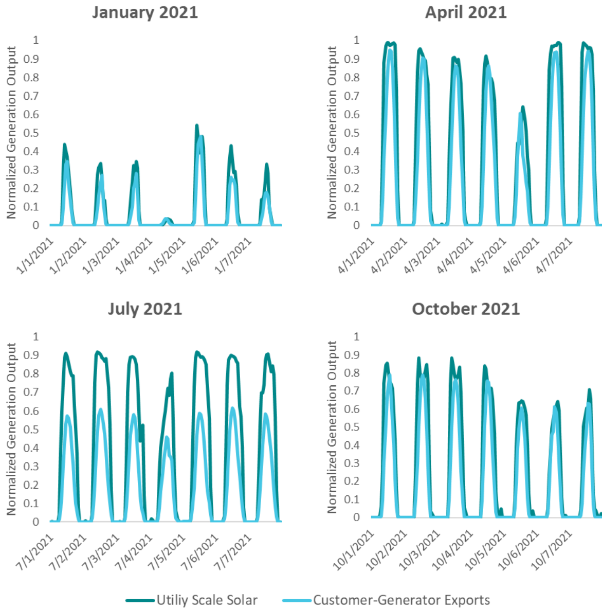
Figure 4.1522 Customer-generator and utility scale solar generation 2021 output normalized for peak generation output
