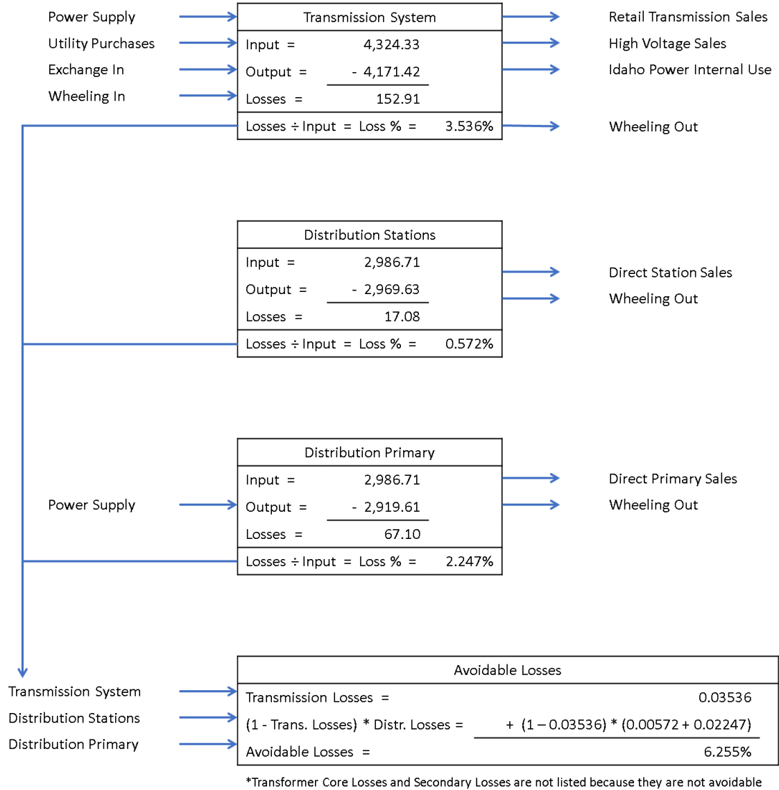
Figure 4.1320 Loss percentage flow diagram (peak hour example)
