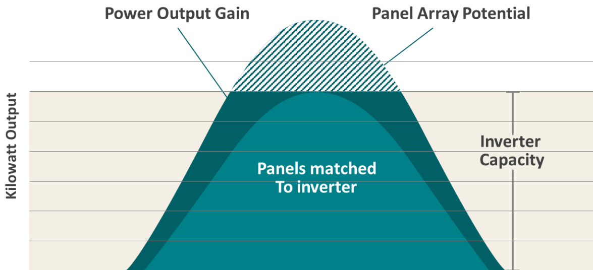
Figure 4.1623 Advantages of higher DC/AC ratio illustration
